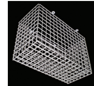
Ceiling Mount Wire Guard Part number: 2530110 Dimensions (mm) L x W x H 407 x 267 x 190
