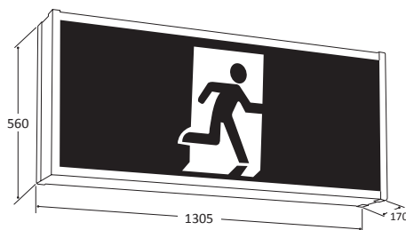
Dimensions (mm)
