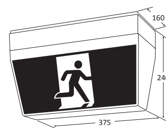
Dimensions (mm) Ceiling Mount
