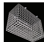
Ceiling Mount Wire Guard Part number: 2530110 Dimensions (mm) L x W x H 407 x 267 x 190
